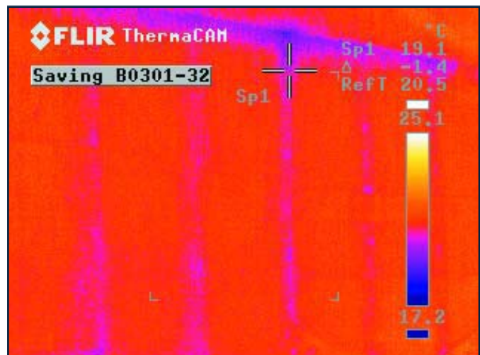
Figure 1a: Thermal photography of stud and batt wall
