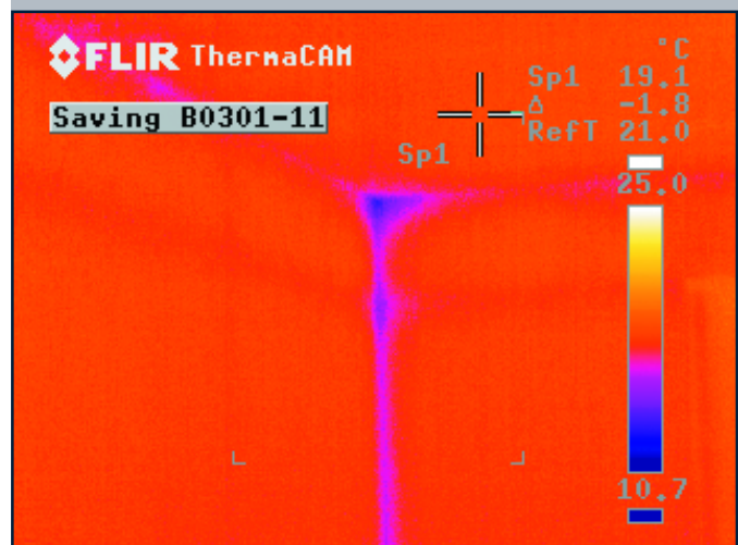
Figure 1b: Thermal photography of SIP wall
