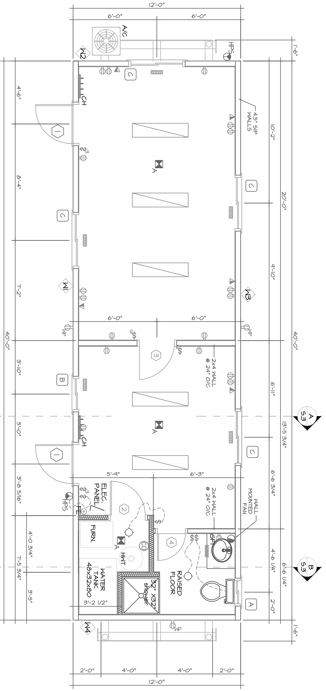
FLOOR PLAN SCALE: 1/4"=1'-0"
